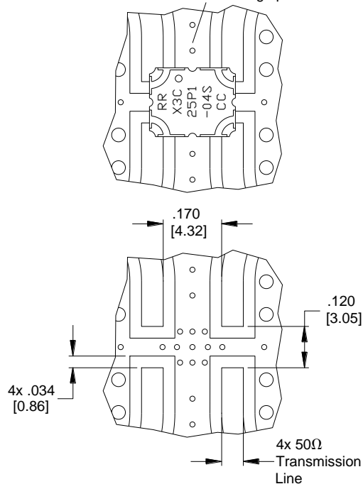
Dimensions are in Inches [Millimeters] X3C25P1-04S Mounting Footprint
